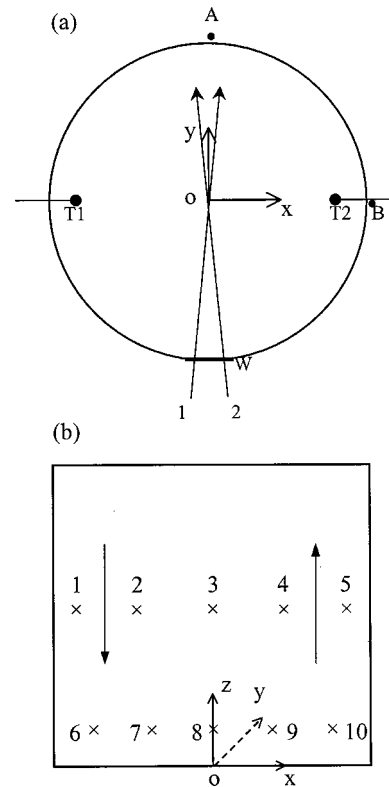
FIG. 1. (a) Schematic diagram of the experimental setup (top view): T1 , T2 , temperature probes; 1, 2, laser beams for LDV; W , optical window. (b) Space coordinates and ten locations for the temperature measurements. The long arrows near the sidewall indicate the direction of the large-scale circulation.
